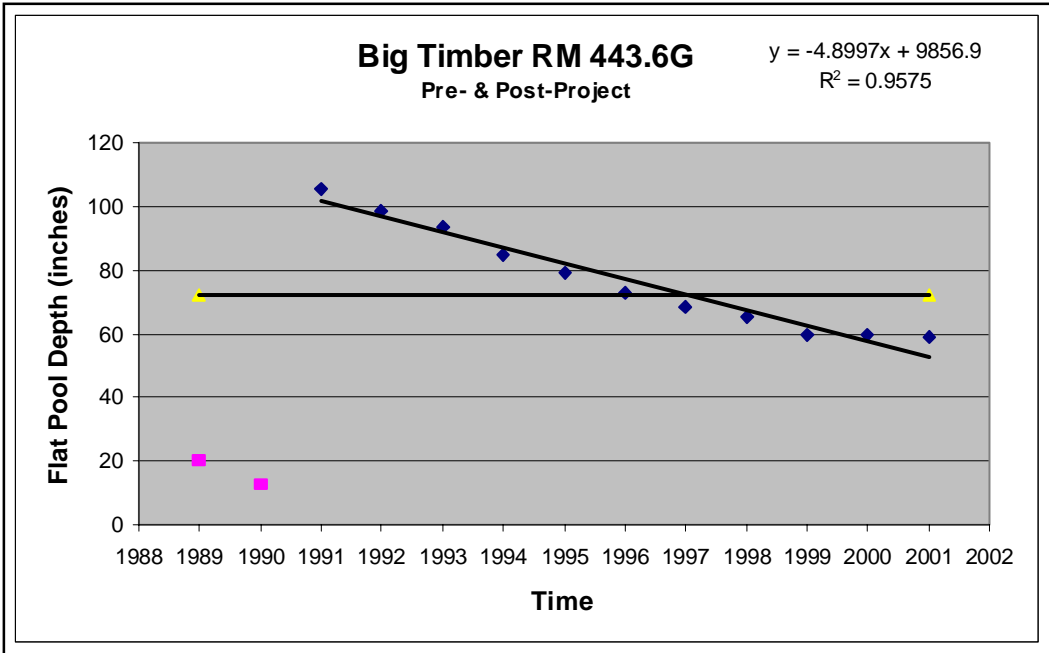
Figure F-1. Sedimentation Rates at Station W-M443.6G
