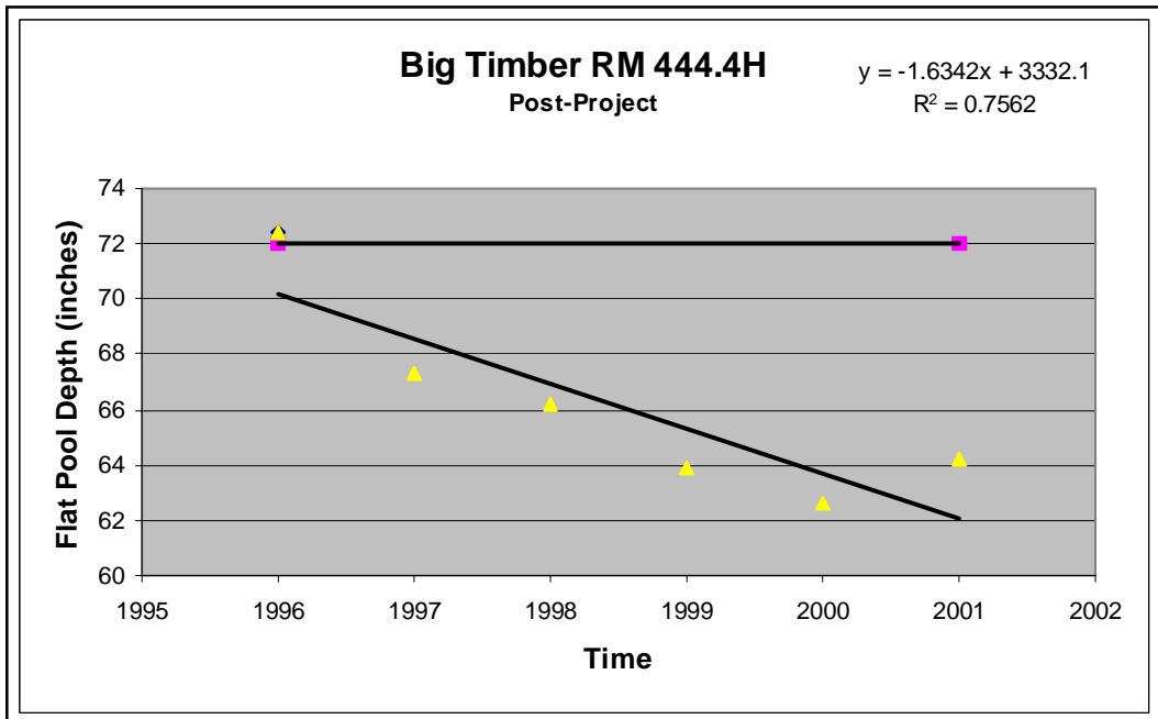
Figure F-2. Sedimentation Rates at Station W-M444.4H
